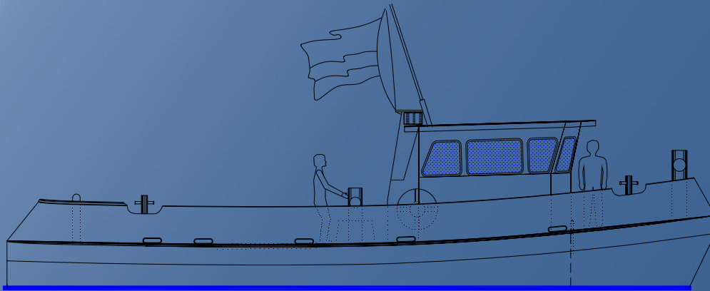
Profile View
